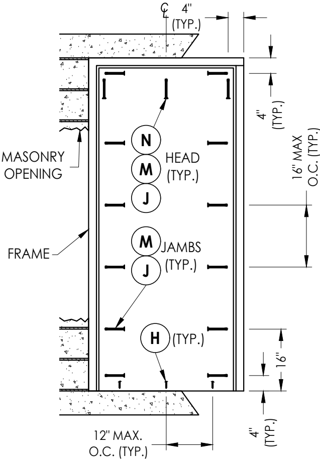
FRAME ANCHORING
